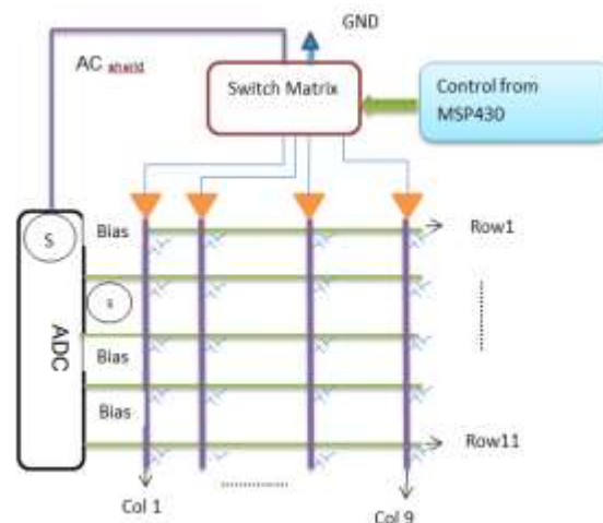
Figure 8: Capacitive sensor array [24]
