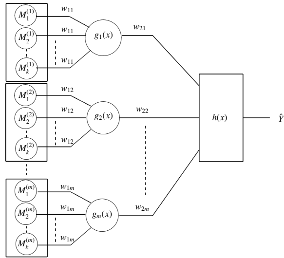
Fig. 1. The multi-layer multi-component predictive system.
