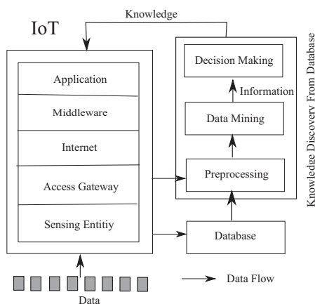
Fig. 8. An architecture of IoT with KDD [41]
