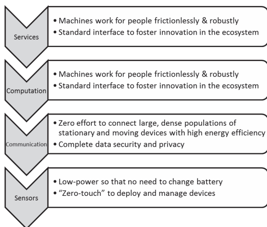
Fig. 3. IoT Challenges [13]
