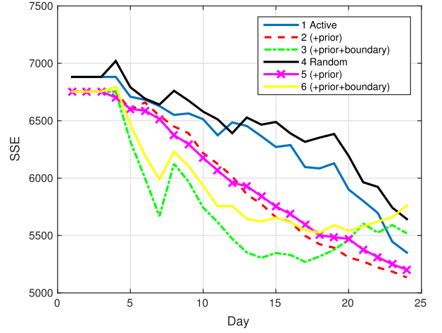
(b) User 2.
