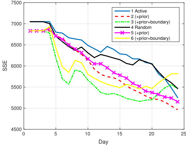
(a) User 1.
