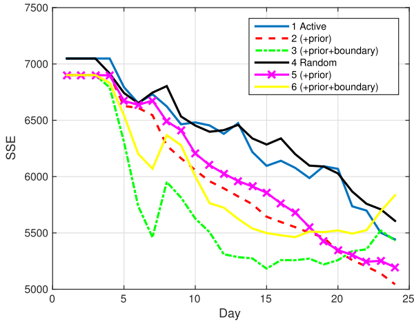
(c) User 3.
