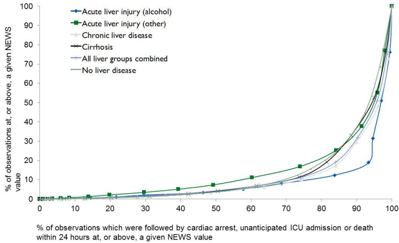
Figure shows the efficiency curves for patients allocated a non-primary diagnosis of acute liver injury due to alcohol, acute liver injury due to other causes, chronic liver disease, cirrhosis, any of the four clinical liver subgroups and patients without any primary or non-primary diagnosis of liver disease. For each NEWS value the percentage of the total number of observations at, or above, that NEWS value is plotted against the percentage of the total number of observations that were followed by cardiac arrest, unanticipated ICU admission or death within 24 hours at, or above, a given NEWS.
