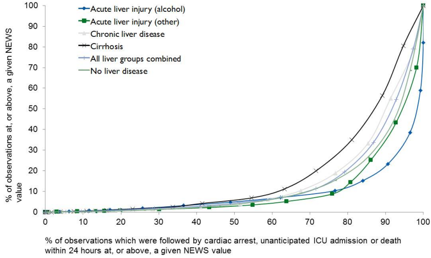
Figure shows the efficiency curves for patients allocated a primary diagnosis of acute liver injury due to alcohol, acute liver injury due to other causes, chronic liver disease, cirrhosis, any of the four clinical liver subgroups and patients without any primary or non-primary diagnosis of liver disease. For each NEWS value the percentage of the total number of observations at, or above, that NEWS value is plotted against the percentage of the total number of observations that were followed by cardiac arrest, unanticipated ICU admission or death within 24 hours at, or above, a given NEWS.
