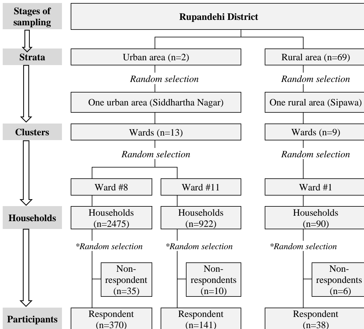
Fig 2: Flowchart of the sampling procedure.
