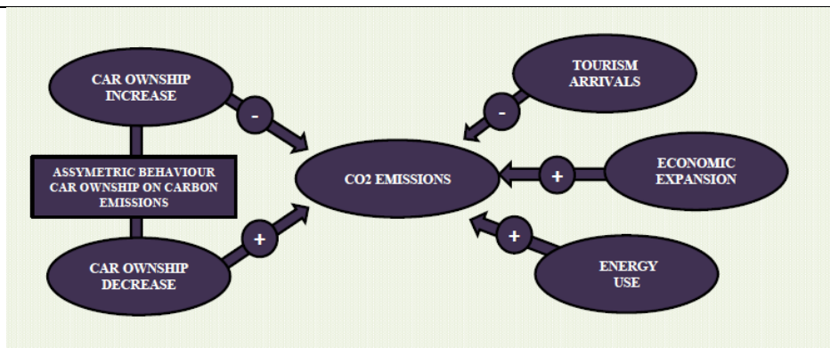
Figure 4: Empirical Results Graphical Abstract
