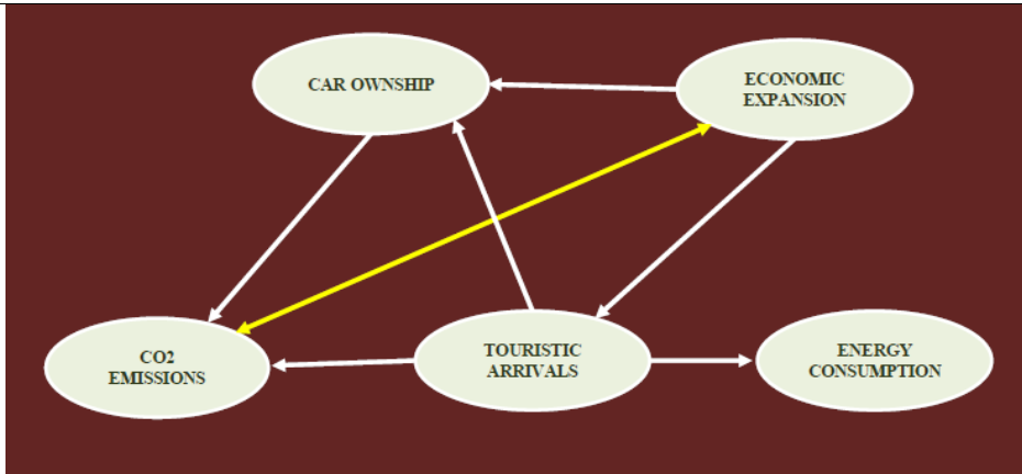
Figure 1: Dicks and Pachenko causality test scheme
