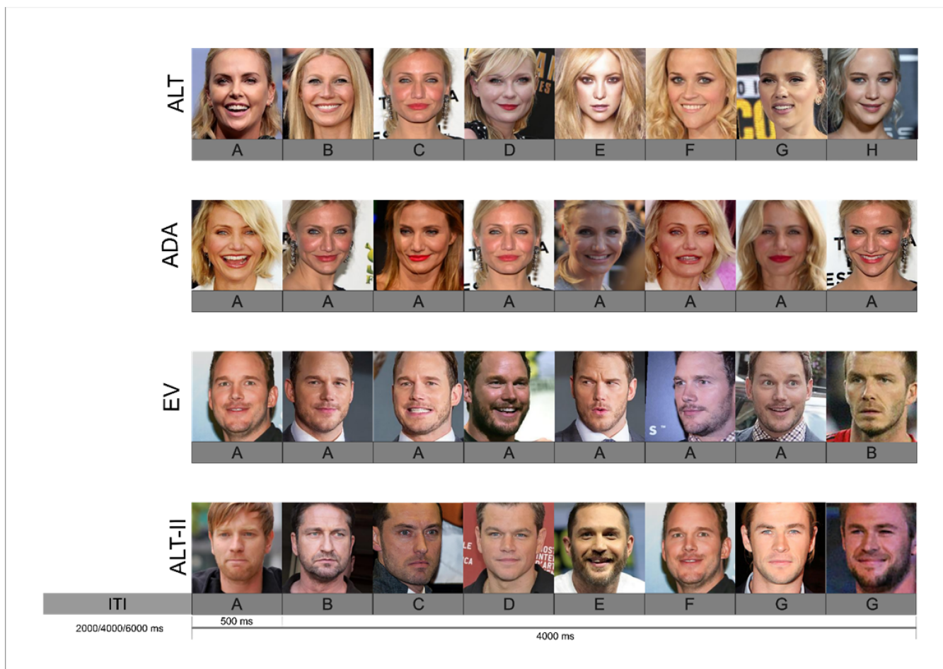
FIGURE 1 Conditions and trial structure in the four applied conditions. Each condition was composed of eight faces. Alternation condition (ALT): different same-sex identities. Adaptation condition (ADA): eight different images of the same identity (ID). Expectation violation condition (EV): seven different images of the same ID, followed by another same-sex ID. ALT-II: six images of different same-sex identities, followed by two different images of another, same-sex ID. Please note that these images are just examples and might not have been part of the actual stimulus set, as we do not have permission for publishing all exemplars we used. All images shown here are subject to either creative commons attribution-share alike license or have no copyrights (public domain)
