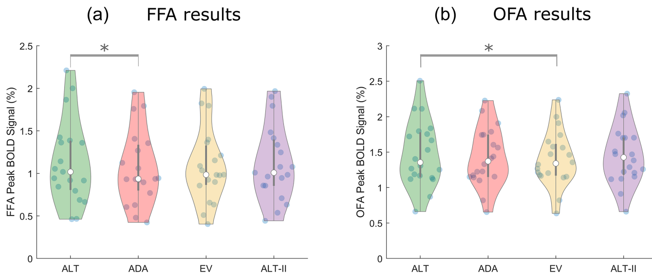
FIGURE 2 Peak blood-oxygen-level dependent (BOLD) signals from individual participants to the different conditions for the bilateral fusiform face area (FFA) (a) and occipital face area (OFA) (b). *represents p < 0.05
