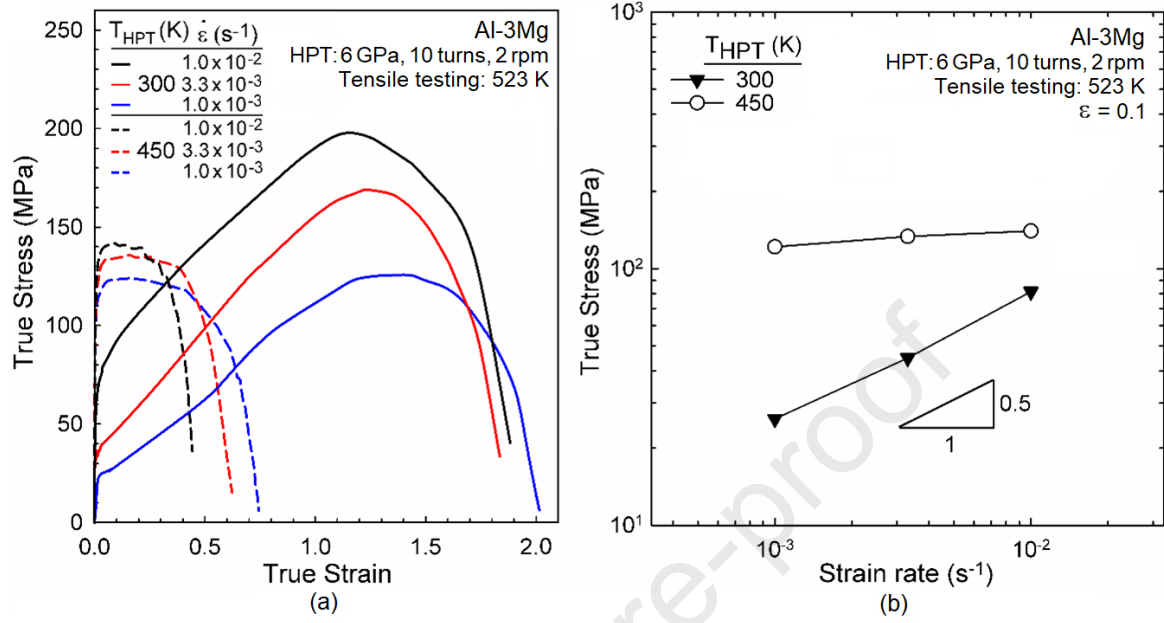
Fig. 7. (a) True stress vs true strain and (b) true stress at \epsilon = 0.1 vs strain rate curves of the Al-3Mg alloy processed by HPT at either 300 or 450 K and subsequently tensile tested at 523 K using strain rates of 1.0 \times 10^{-2} , 3.3 \times 10^{-3} and 1.0 \times 10^{-3} s ^{-1} .
