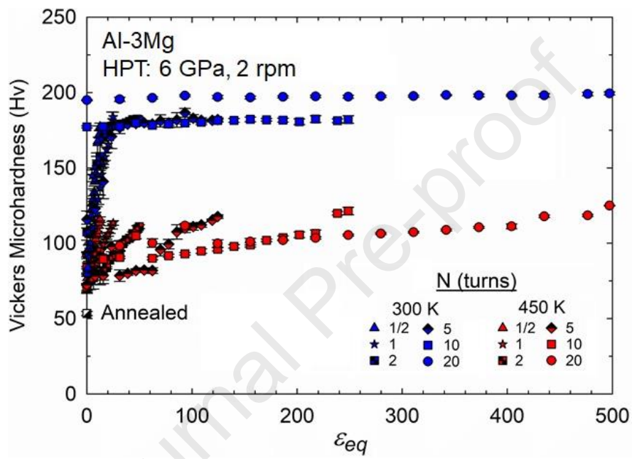
Fig. 10. Vickers microhardness as a function of equivalent strain for the Al-3Mg alloy processed by HPT at either 300 or 450 K.
