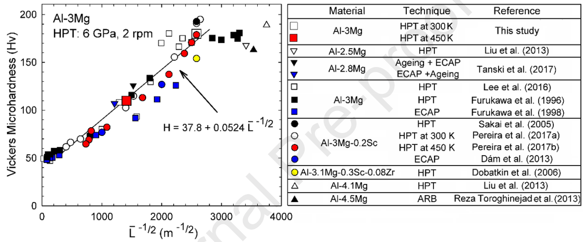
Fig. 11. Vickers microhardness as a function of \bar{L}^{-1/2} for Al-Mg alloys with similar compositions subjected to either HPT [16,21,48,49,65,69,91,92], ECAP [39,90,93] and ARB [94] at different processing conditions.
