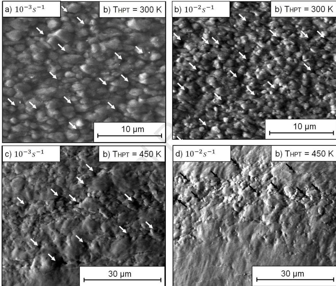
Fig. 9. SEM images taken along the gauge area of Al-3Mg specimens processed through 10 turns of HPT at either (a and b) 300 or (c and d) 450 K and further tested in tension at 523 K at strain rates of 10^{-3} and 10^{-2} s^{-1} .
