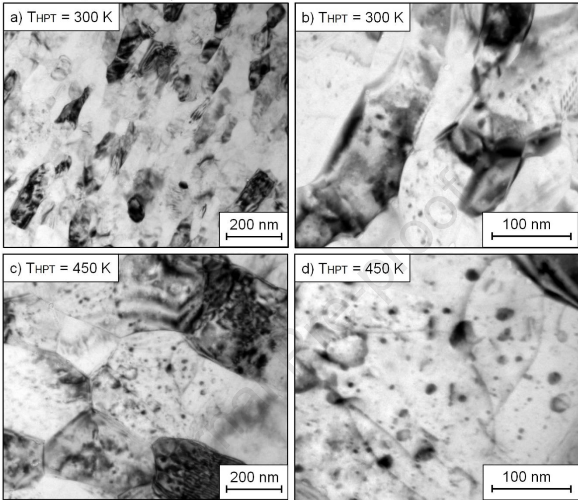
Fig. 5. TEM images revealing the presence of precipitates for the Al-3Mg alloy processed by 10 turns of HPT at either (a and b) 300 or (c and d) 450 K.
