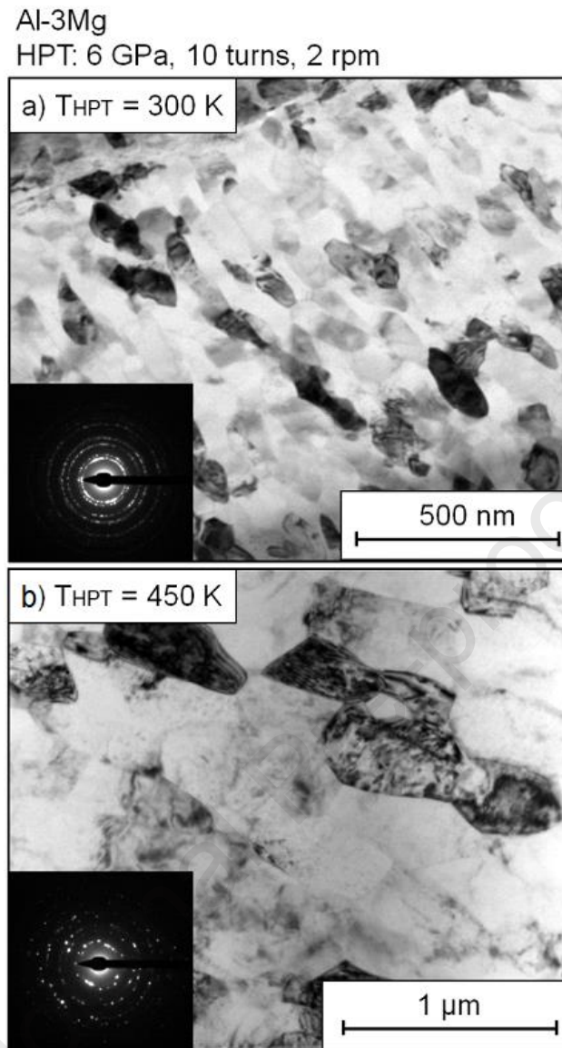
Fig. 4. TEM images and corresponding SAED patterns showing grains and dislocation structures of the Al-3Mg alloy processed by 10 HPT turns at either (a) 300 or (b) 450 K.
