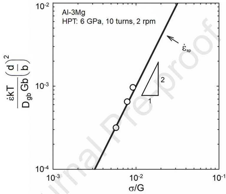
Fig. 12. Temperature and grain size compensated strain rate as a function of normalized stress for the Al-3Mg alloy processed by HPT at 300 K and tensile tested at 523 K: the solid line corresponds to the theoretical prediction for superplastic flow [97].
