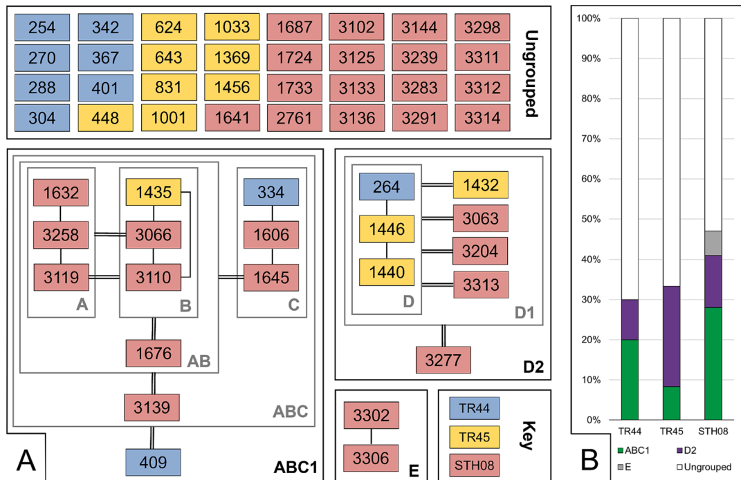
Fig. 14. (A) 'Family tree' of Stonehenge fragments showing how the compositional overlap between single samples can be used to define compositional continua (families). Single lines indicate where a geochemical match exists between individual fragments. Double lines indicate where a geochemical match exists between a continuum and a single fragment. Rectangles enclose compositional continua. The iterative processes described in the text yield three compositional continua (families): ABC1, D2 and E. The samples that did not overlap any remain ungrouped. (B) Column chart showing the proportion of the three compositional families (and ungrouped fragments) present in the assemblages from the three excavated areas.
