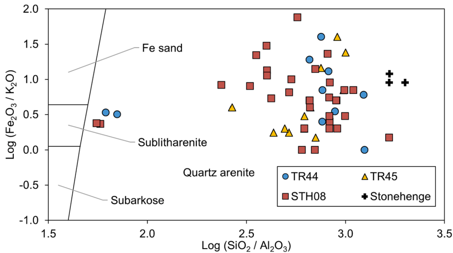
Fig. 9. Log (SiO 2 / Al 2 O 3 ) vs. Log (Fe 2 O 3 / K 2 O) data for sarsen fragments, differentiated by excavation, alongside equivalent data from the interior of Stone 58 at Stonehenge (Nash et al., 2020). Axes modified after Herron (1988)..
