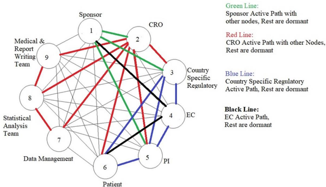
Fig. 3. Private channels on the Hyperledger fabric pluggable architecture.
