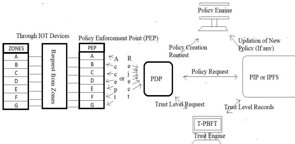
Fig. 18. Process of policy decision points (PDPs) and policy enforcement points (PEPs).
