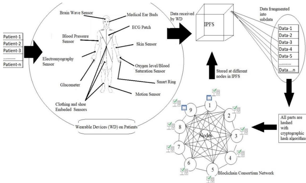
Fig. 17. Storage of wearable device data through IPFS
