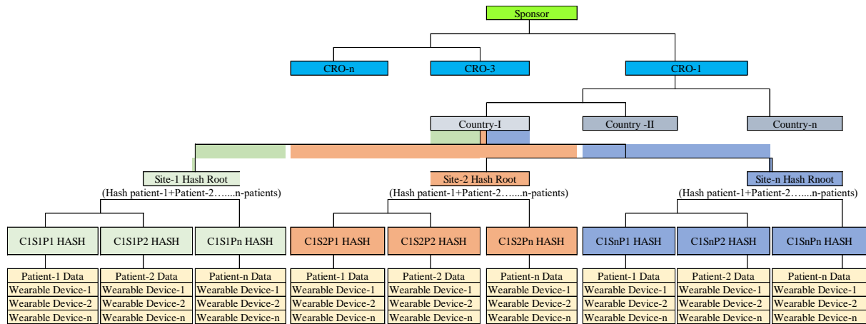
Fig. 11. Patient-based Merkle tree of the country.
