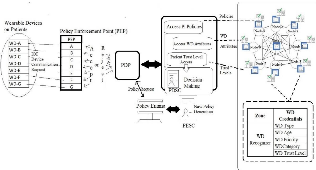
Fig. 16. ABAC access policy mechanism implementation in z-TAB.
