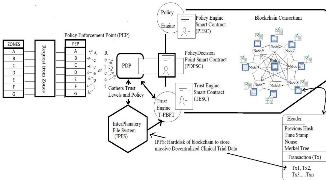
Fig. 14. Zero-trust architecture blockchain (z-TAB) model.
