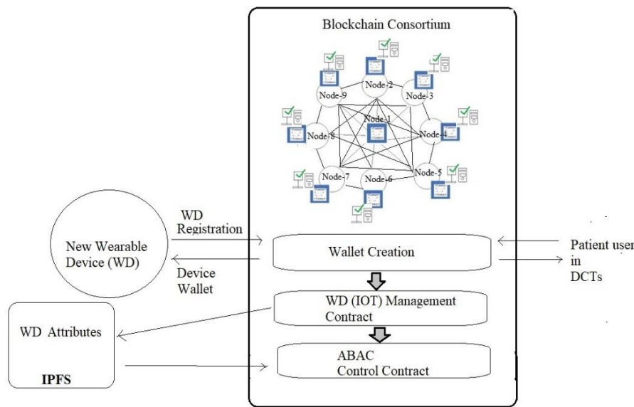
Fig. 15. Registration of wearable devices on blockchain.
