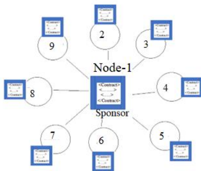
Fig. 8. Code replication on DCT stakeholder's nodes
