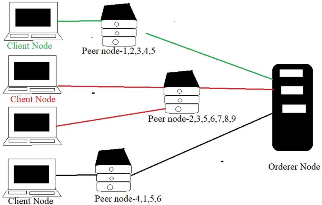
Fig. 4. Hyperledger fabric system architecture [42].
