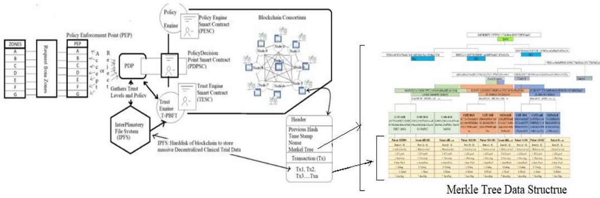
Fig. 22. Blockchain, wearable devices, and data storage on IPFS.
