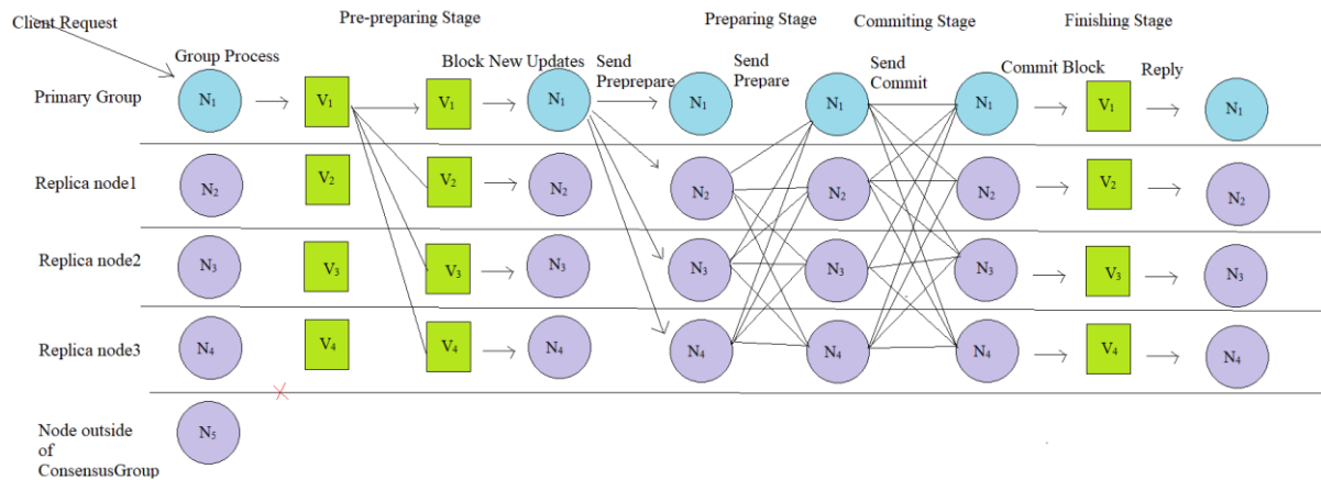
Fig. 13. Propagation of the consensus process in T-PBFT [56].
