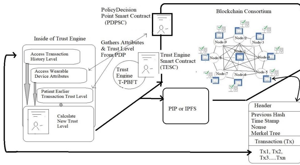
Fig. 19. Trust engine on blockchain.
