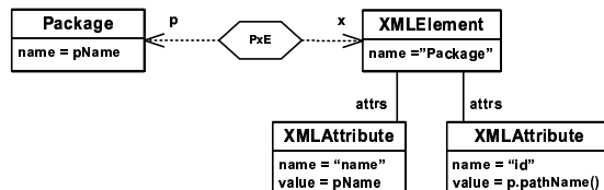
Fig. 8. A UML package to XML relation
