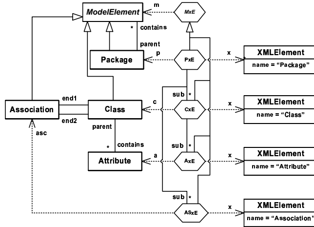
Fig. 10. Transformation composition
