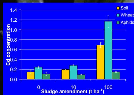
Figure 1. Cadmium concentrations (mg kg -1 ) in soil, wheat shoots and grain aphids following the amendment of soil with sewage sludge (mean ± 1 SE).
