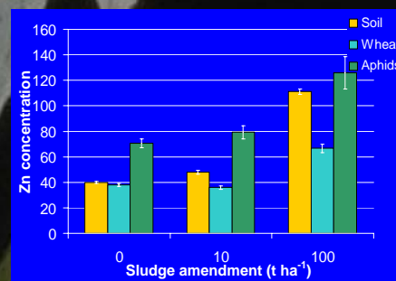
Figure 2. Zinc concentrations (mg kg -1 ) in soil, wheat shoots and grain aphids following the amendment of soil with sewage sludge (mean ± 1 SE).
