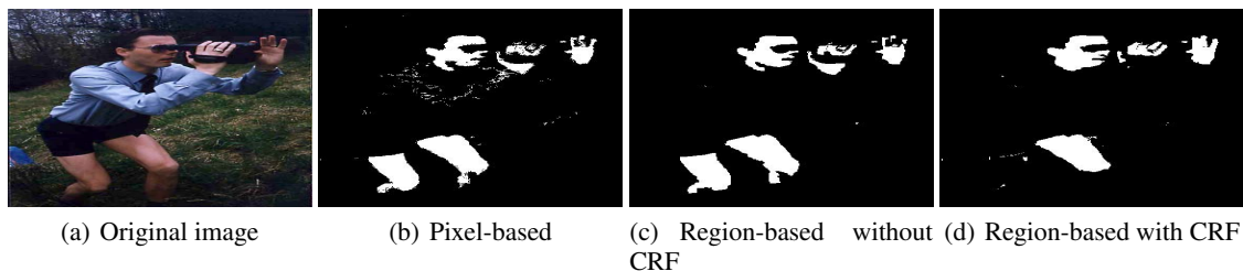
Figure 3: This example shows the advantages of the region-based approach even without CRF (see sub figures b and c). Sub figures c and d show the failure case when CRF is applied.
