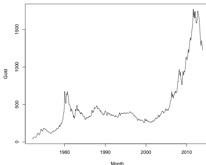
Figure 1: Time series for Gold price (January 1972 - December 2013).
