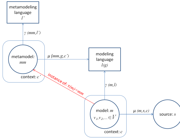
Fig. 2. Metamodeling.
