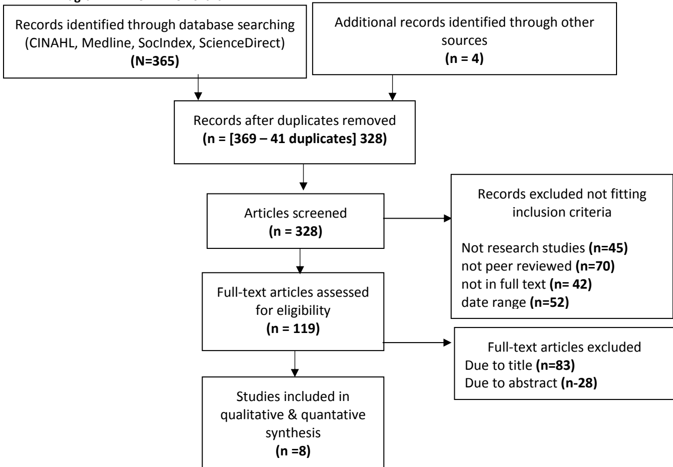
Diagram 1: PRISMA flowchart
