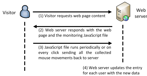
Fig. 4. Mouse movement collection process.
