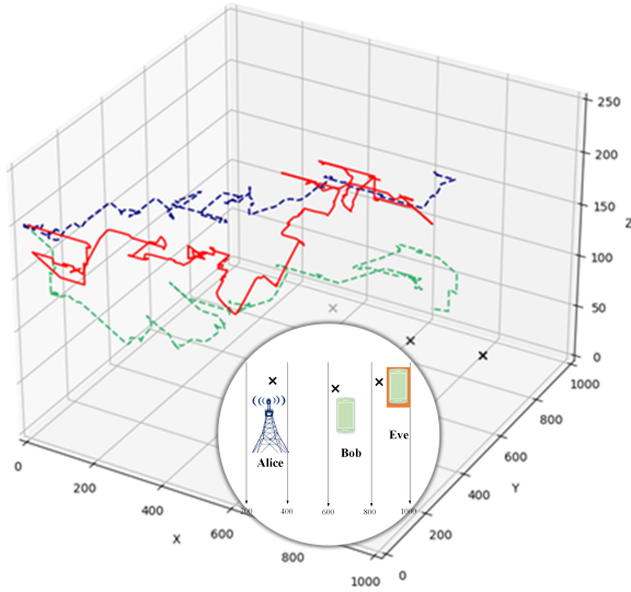
Fig. 3. The 3D UAV trajectory.
