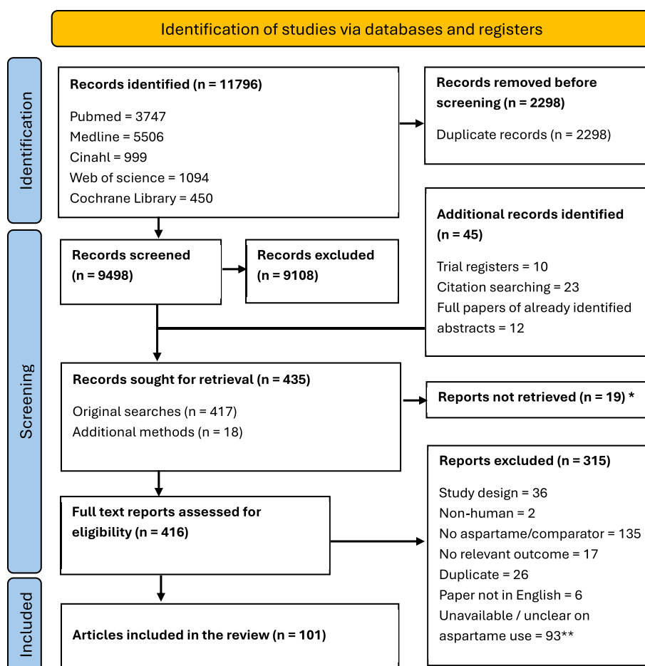
FIGURE 1. PRISMA diagram. * Includes article record not found (n = 7), full study article not available (n = 11), and article not retrieved due to copyright (n = 1). ** Where data on aspartame use was unavailable or unclear, clarification was sought from authors. Studies were only included if authors responded by the September 30, 2024, with confirmation of aspartame use. PRISMA, Preferred Reporting Items for Systematic Reviews and Meta-Analyses.
